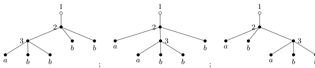
Figure 4 Planted ternary increasing plane trees on [3] encoded by ab^4D_{G_3} and a^2b^3D_{G_3}
