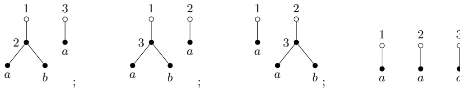
Figure 3 Three 2-forests on [3] encoded by a^2 b D_{G_2}^2 , and the 3-forest on [3] encoded by a^3 D_{G_2}^3
